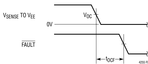
Figure 3. Open-Circuit Filter Timing
