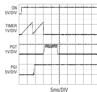
Power-Up Waveforms
