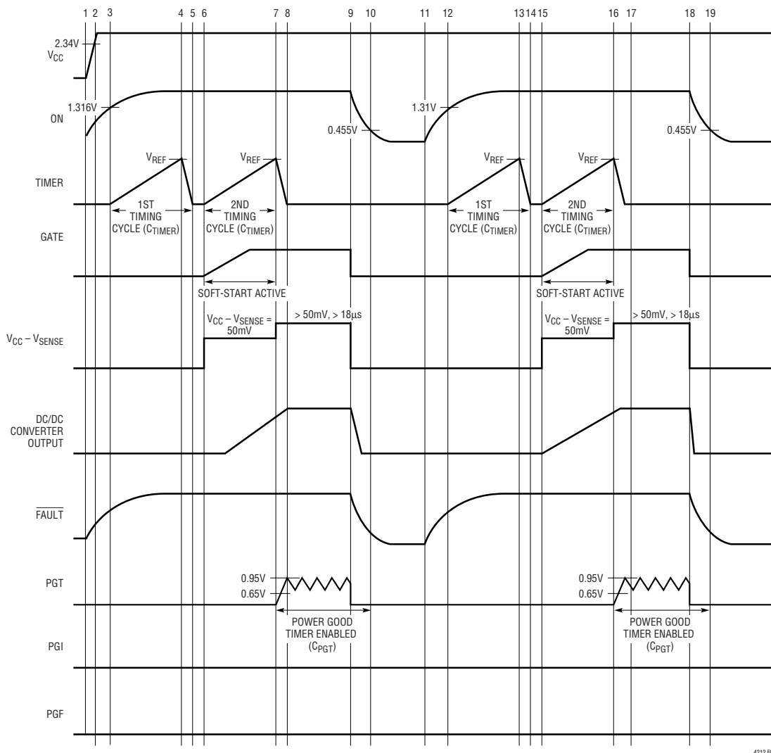
Figure 6. Autoretry Sequence
