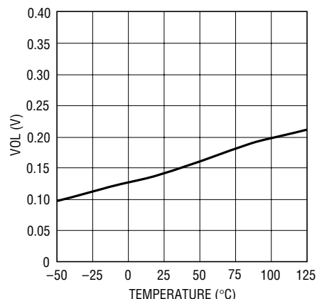
FAULT V_{OL} vs Temperature
