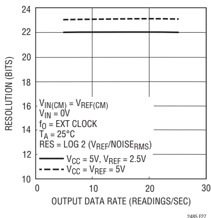
Figure 27. Resolution ( \text{Noise}_{\text{RMS}} \leq 1\text{LSB} ) vs Output Data Rate and Reference Voltage
