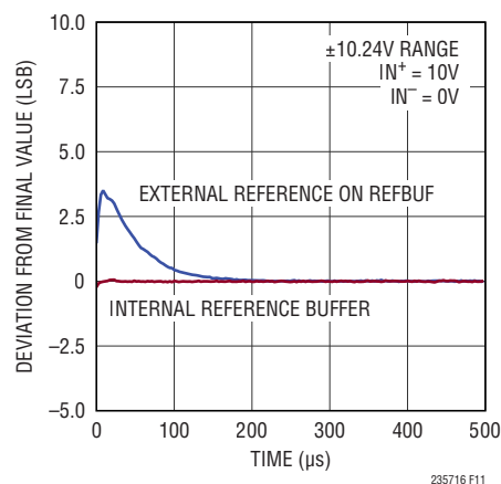
Figure 11. Burst Conversion Response of the LTC2357-16, f_{\text{SMPL}} = 350\text{kps}
