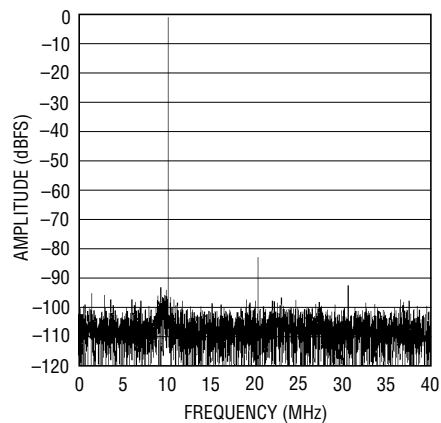
8192 Point FFT, f_{IN} = 250.2\text{MHz} , -1dB, PGA = 1
