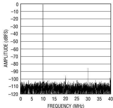
8192 Point FFT, f_{IN} = 70.2\text{MHz} , -1dB, PGA = 0
