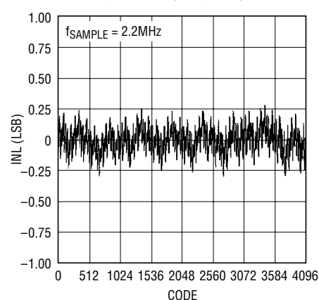
Integral Nonlinearity vs Output Code (Unipolar)
