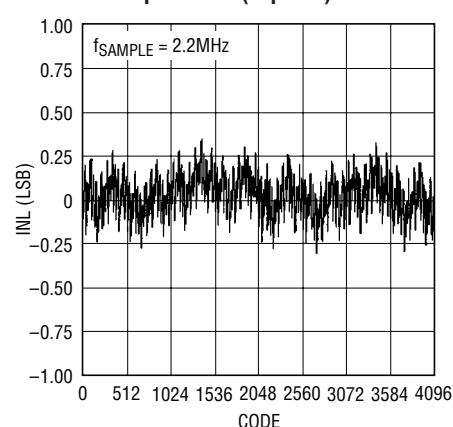
Integral Nonlinearity vs Output Code (Bipolar)
