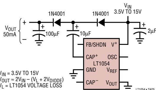
Positive Doubler
