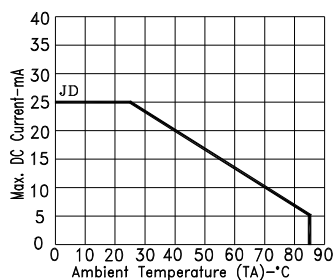
Fig5. MAX. ALLOWABLE DC CURRENT VS. AMBIENT TEMPERATURE.
