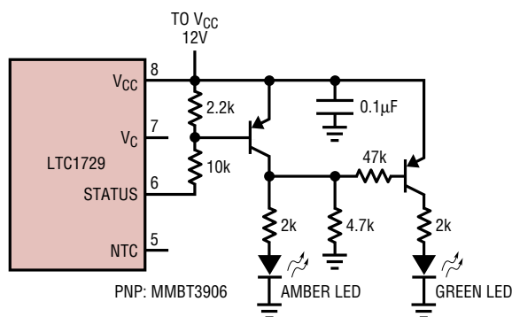
Using STATUS Pin to Indicate Charge Status
