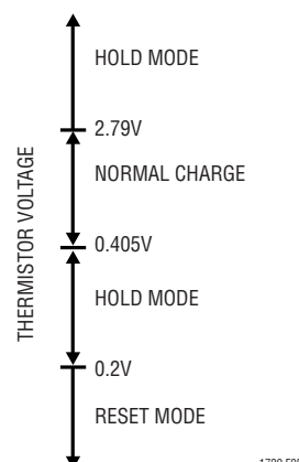
Figure 5. NTC Voltage Operating Range
