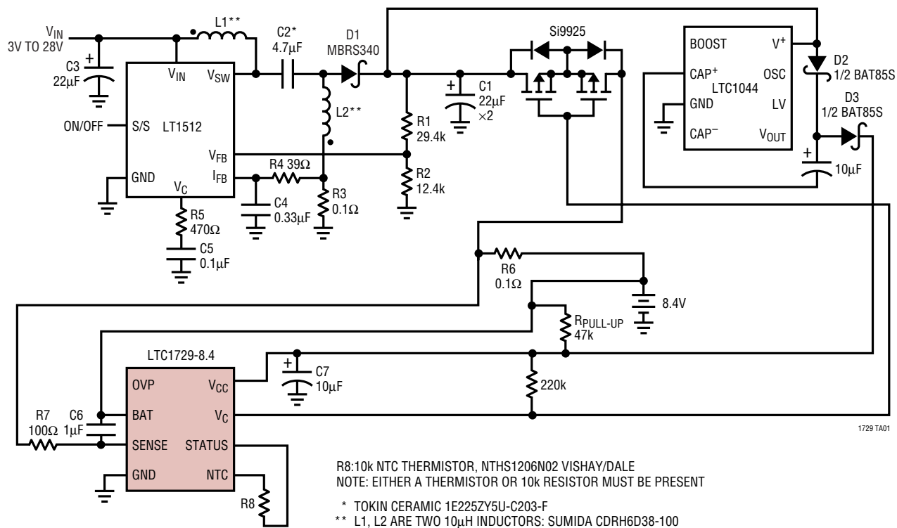
Wide Input Voltage Range 1A Charger
