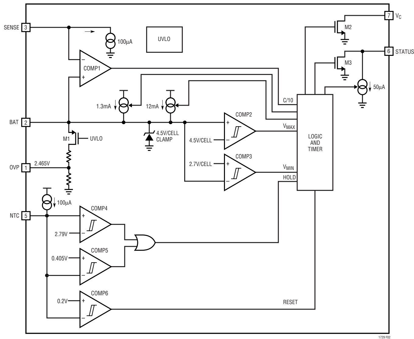
Figure 2. Block Diagram
