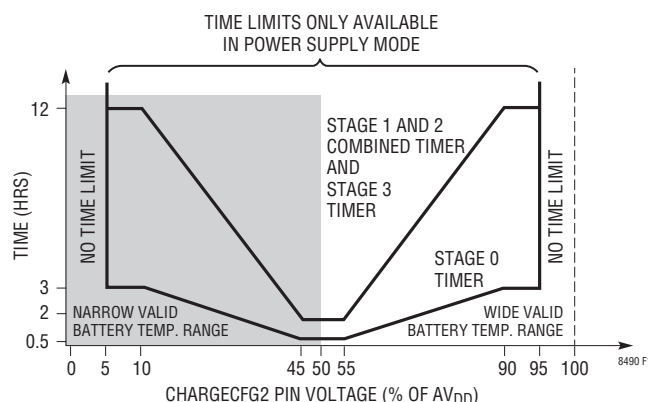
Figure 14. CHARGECONFIG2 Pin Voltage Settings
