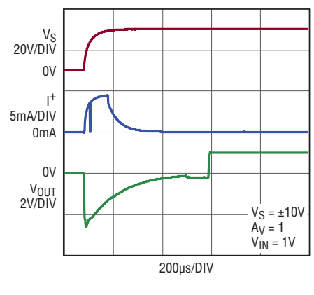
Start-Up Response
