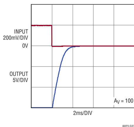
Positive Output Overdrive Recovery
