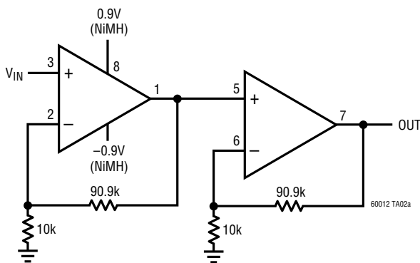
Gain of 100 Amplifier (400kHz GBW on 30 \mu A Supply)
