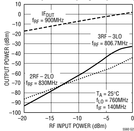
IFOUT, 2 x 2 and 3 x 3 Spurs vs RF Input Power (Single Input Tone)
