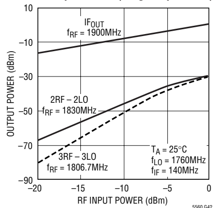
IF OUT , 2 × 2 and 3 × 3 Spurs vs RF Input Power (Single Input Tone)
