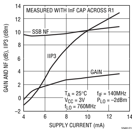
Figure 15. 900MHz Downconverting Mixer Gain, Noise Figure and IIP3 vs Supply Current
