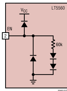
Figure 12. Enable Input Circuit
