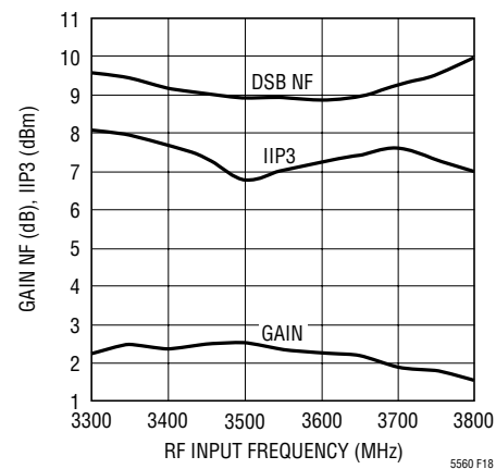
Figure 18. LT5560 Performance as a 3600MHz Downconverting Mixer
