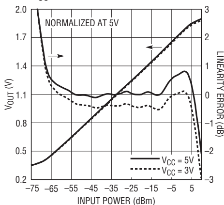
Output Voltage, Linearity Error vs VCC @40MHz
