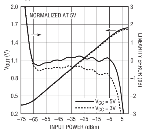
Output Voltage, Linearity Error vs VCC @2140MHz
