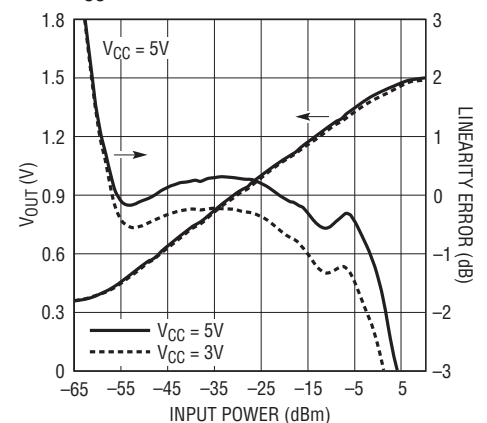
Output Voltage, Linearity Error vs VCC @3600MHz
