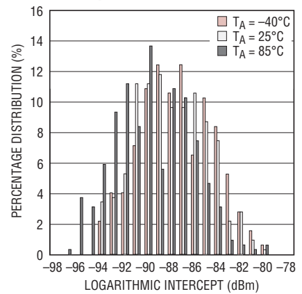
Logarithmic Intercept Distribution vs Temperature at 2.14GHz
