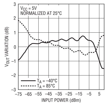
VOUT Variation vs Input Power at 2.14GHz
