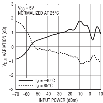
VOUT Variation vs Input Power at 3.6GHz
