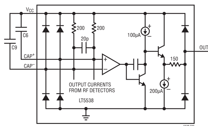
Figure 3. Simplified Schematic of the Output Interface
