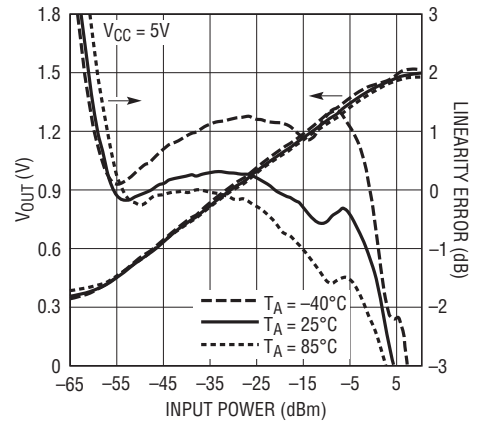
Output Voltage, Linearity Error vs Input Power at 3.6GHz
