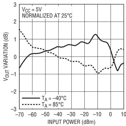
VOUT Variation vs Input Power at 2.7GHz
