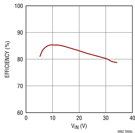
SEPIC Efficiency vs Input Voltage
