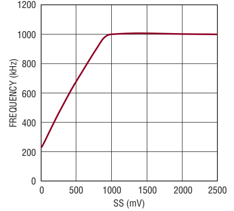
Soft-Start/Track vs Frequency (1MHz)
