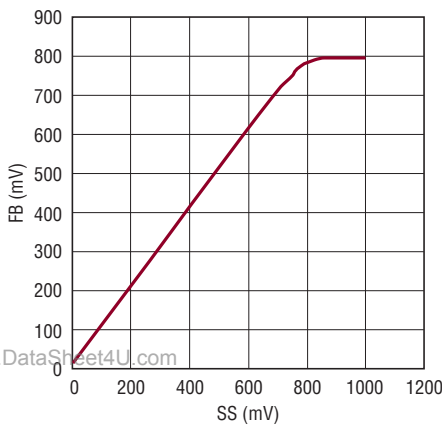
Soft-Start/Track vs V_{FB}
