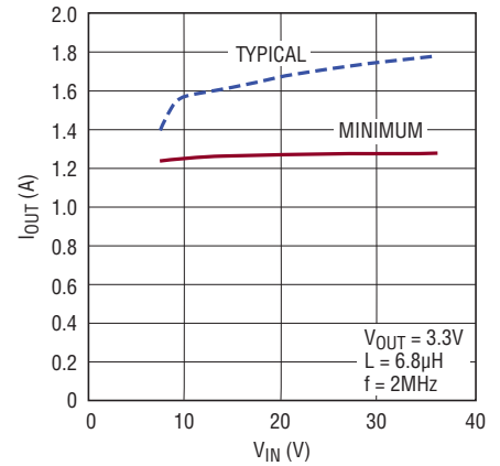
3.3V OUT Maximum Load Current
