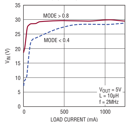
5V OUT Maximum V_{IN} for Full Frequency (2MHz)
