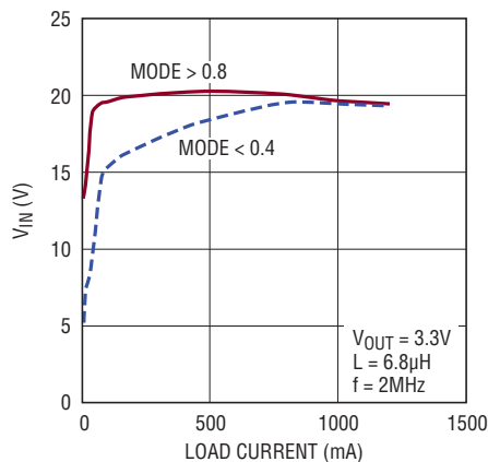
3.3V OUT Maximum V_{IN} for Full Frequency (2MHz)
