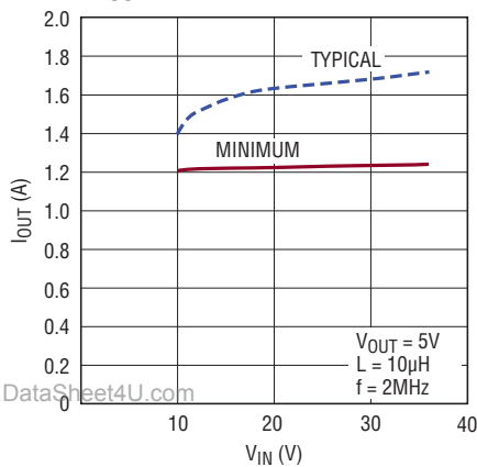
5V OUT Maximum Load Current
