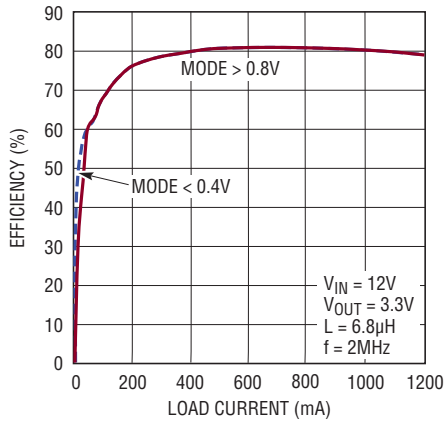
3.3V OUT Efficiency (2MHz)
