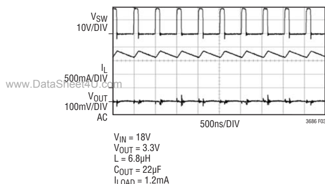
Figure 3. Continuous Mode Operation Near Minimum On Time
