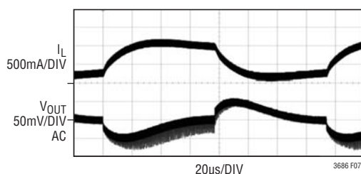
Figure 7. Transient Load Response of the LT3686 with Different Output Capacitors as the Load Current Is Stepped from 0.25A to 1A. V_{IN} = 12V , V_{OUT} = 3.3V , L = 6.8\mu H , Frequency = 2MHz
