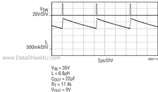
Figure 13. The LT3686 Reduces its Frequency from 2MHz to 160kHz to Protect Against Shorted Output
