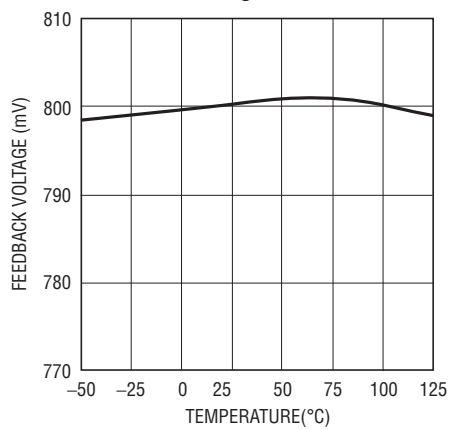
Feedback Voltage
