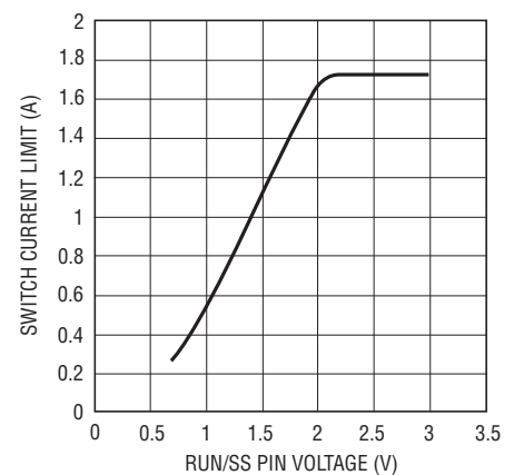
Soft-Start
