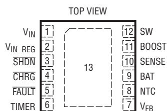
DD PACKAGE 12-LEAD (3mm × 3mm) PLASTIC DFN T_{JMAX} = 125^{\circ}C , \theta_{JA} = 43^{\circ}C/W , \theta_{JC} = 3^{\circ}C/W EXPOSED PAD (PIN 13) IS GND, MUST BE SOLDERED TO PCB
