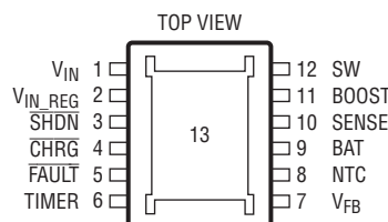
MSE PACKAGE 12-LEAD PLASTIC MSOP T_{JMAX} = 125^{\circ}C , \theta_{JA} = 43^{\circ}C/W , \theta_{JC} = 3^{\circ}C/W EXPOSED PAD (PIN 13) IS GND, MUST BE SOLDERED TO PCB
