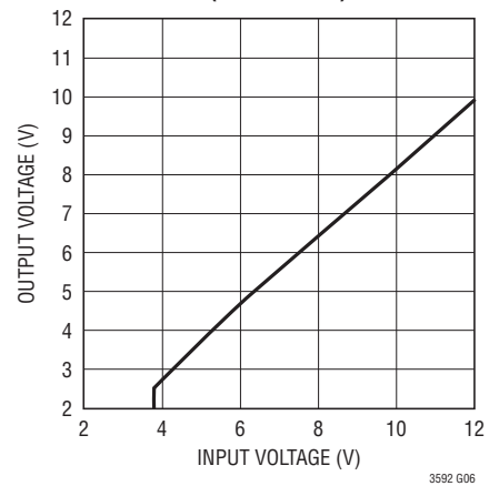
Minimum V_{IN} for 500mA Output Current vs V_{OUT} , L = 6.8\mu\text{H} , f = 900\text{kHz} (LED Loads)
