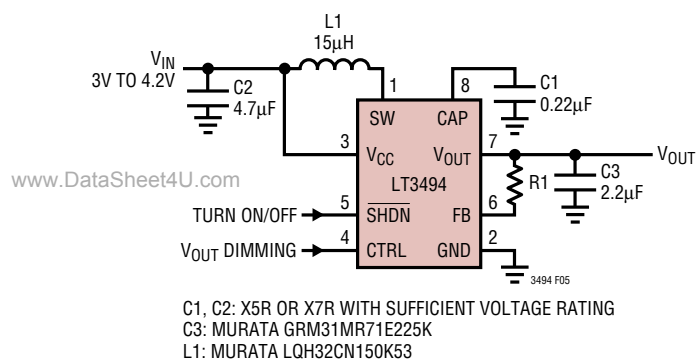
Figure 5. One Li-Ion Cell Input Boost Converter with the LT3494
