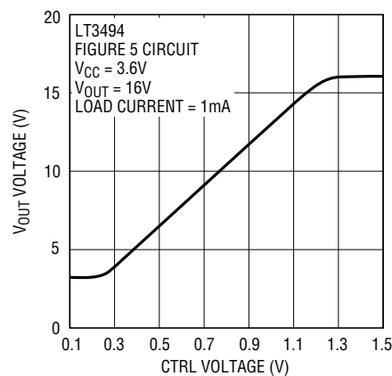
V_{\text{OUT}} vs CTRL Voltage
