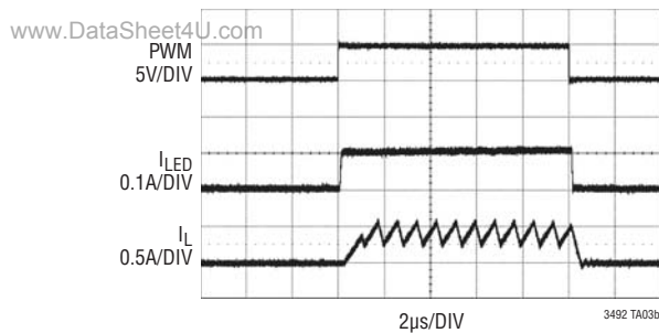
1000:1 PWM Dimming at 100Hz
