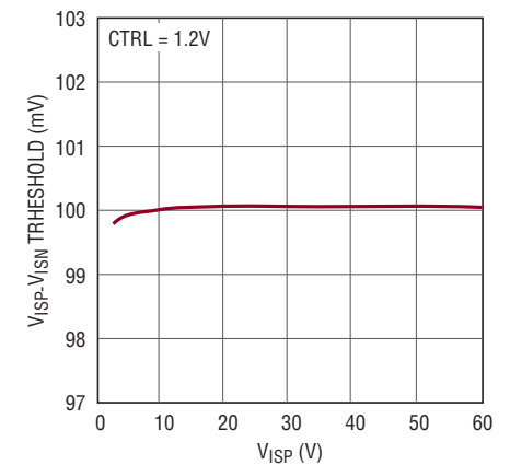
V_{ISP}-V_{ISN} Threshold vs V_{ISP}
