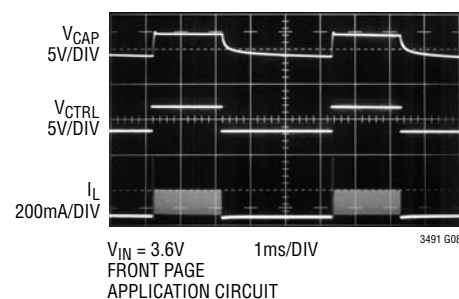
Transient Response
