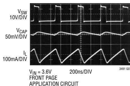
Switching Waveform
