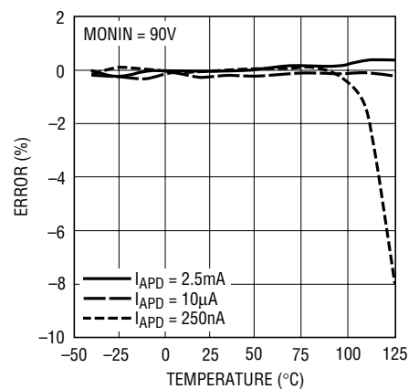
APD Current Monitor Accuracy vs Temperature
