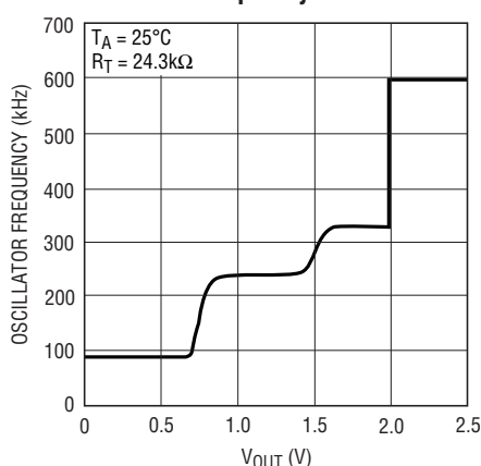
Oscillator Frequency Foldback
