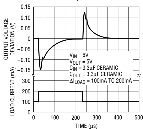
Transient Response
