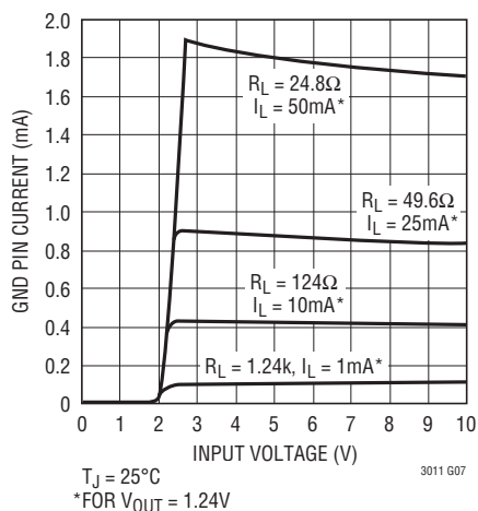
GND Pin Current
