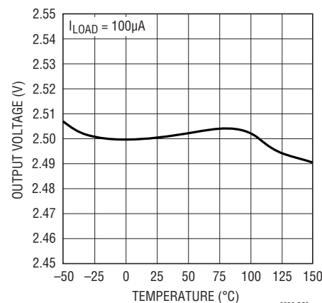
Output Voltage LT3009-2.5
