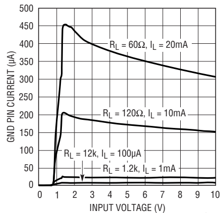
GND Pin Current LT3009-1.2
