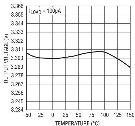
Output Voltage LT3009-3.3
