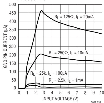
GND Pin Current LT3009-2.5
