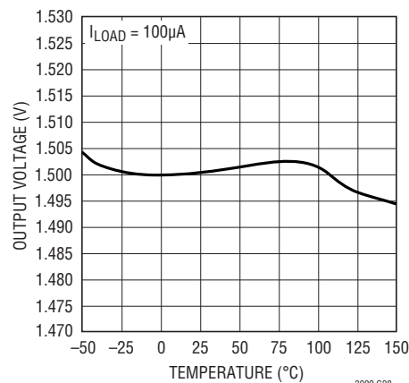
Output Voltage LT3009-1.5
