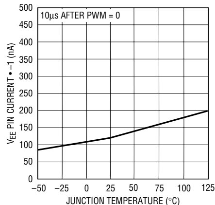
V_{\text{EE}} Pin Current (Out of the Pin) vs Temperature
