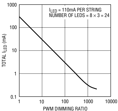
PWM Dimming
