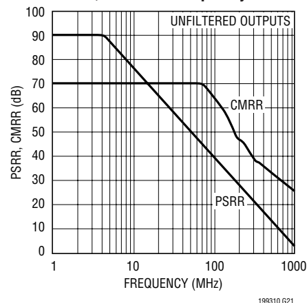
PSRR, CMRR vs Frequency
