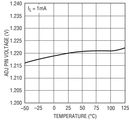
LT1761-BYP, LT1761-SD ADJ Pin Voltage
