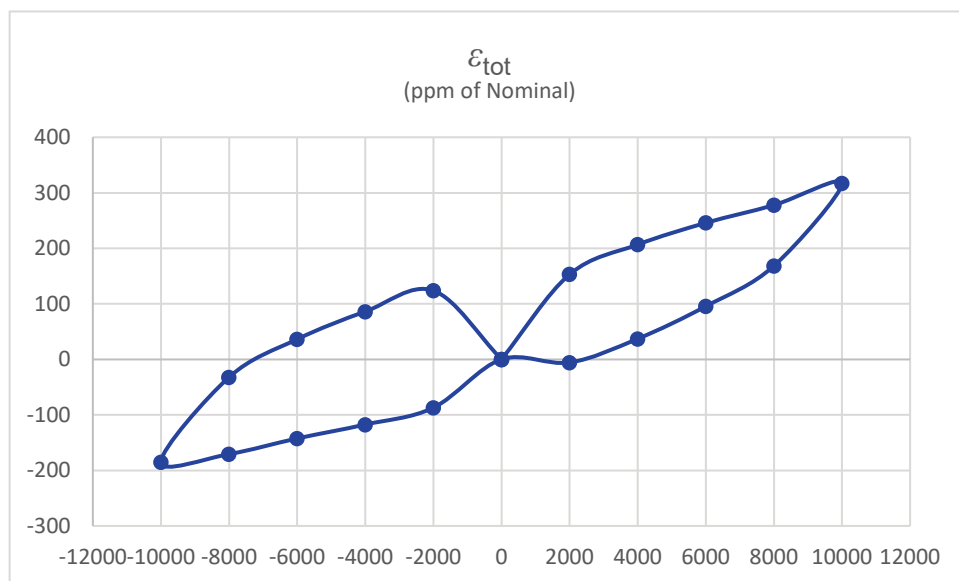
Figure 3: \varepsilon_{\text{tot}} @ 25 °C, U_C = \pm 60 V with R_M = 0.1 \Omega
