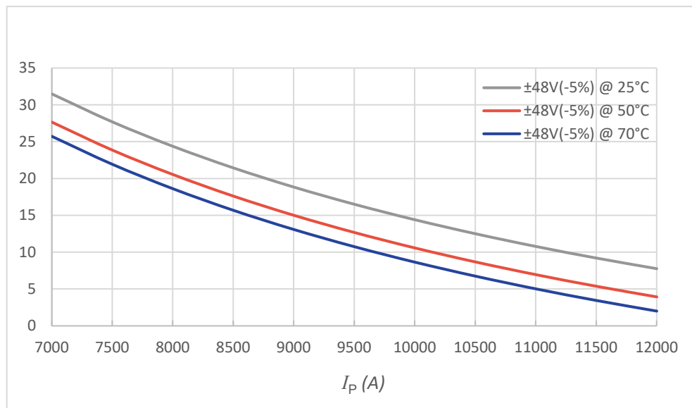
Figure 1: Maximum measuring resistance @ ±48 V
