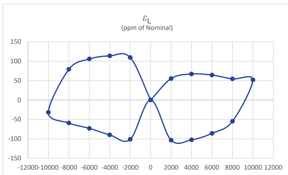
Figure 4: \varepsilon_L @ 25 °C, U_C = \pm 60 V with R_M = 0.1 \Omega
