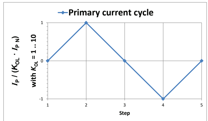
Figure 6: Current cycle used to measure magnetic and electrical offset (transducer supplied)
