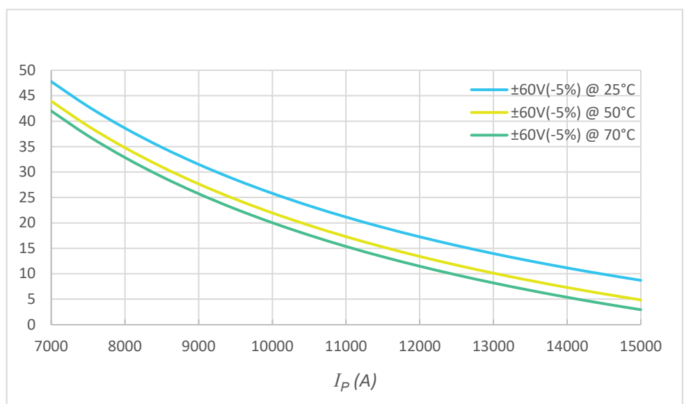
Figure 2: Maximum measuring resistance @ ±60 V
