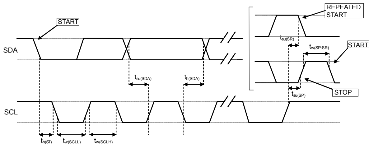
Figure 9. I 2 C slave timing diagram
