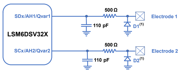
Figure 29. Qvar external connections to pin 2, 3 (Qvar input)
