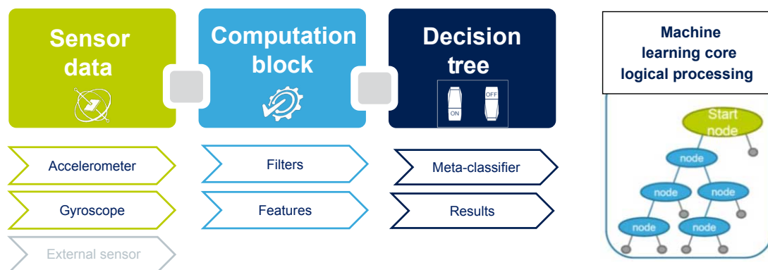
Figure 4. Machine learning core in the LSM6DSV32X
