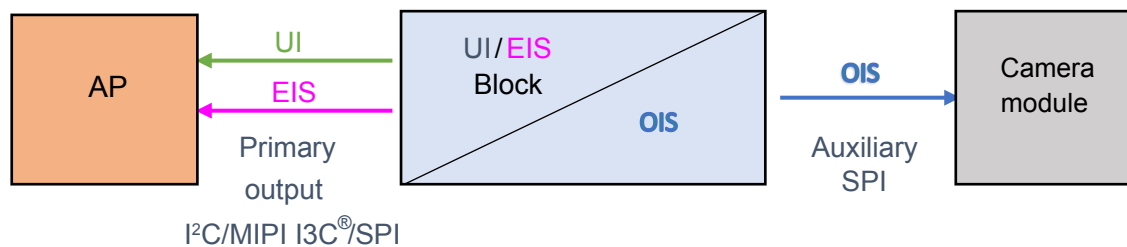
Figure 24. LSM6DSV32X supports UI, enhanced EIS, and OIS processing simultaneously
