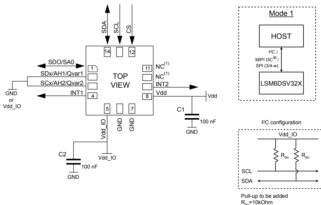
Figure 28. LSM6DSV32X electrical connections in mode 1
