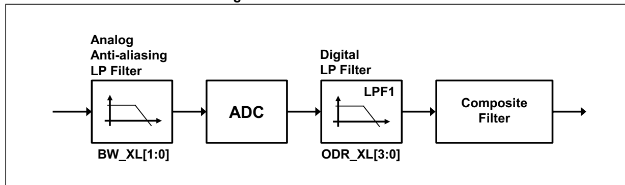
Figure 6. Accelerometer chain
