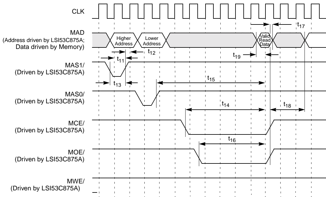
Figure 6.31 \leq 64 Kbytes ROM Read Cycle
