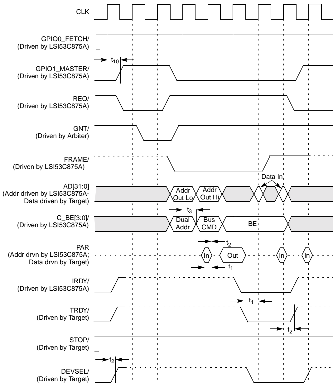
Figure 6.20 Burst Read, 64-Bit Address and Data
