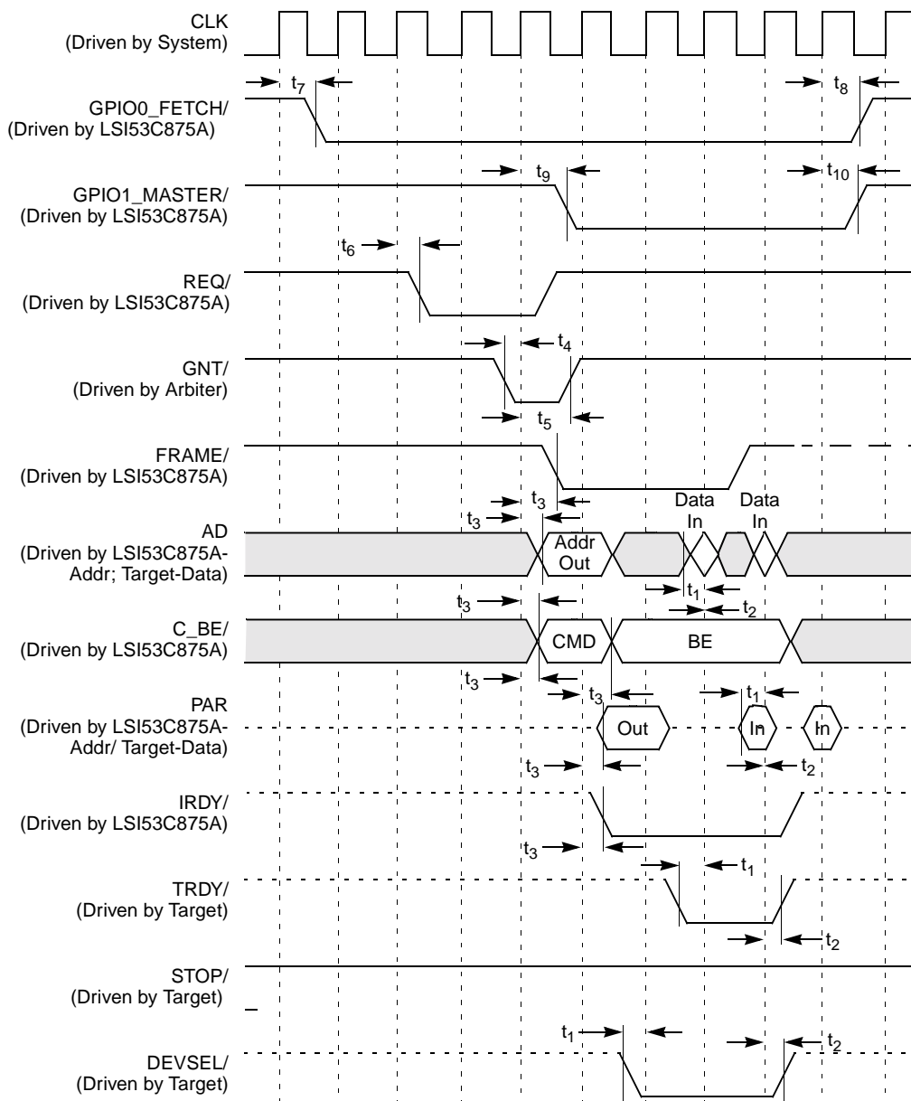
Figure 6.16 Burst Opcode Fetch, 32-Bit Address and Data
