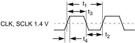
Figure 6.6 External Clock
