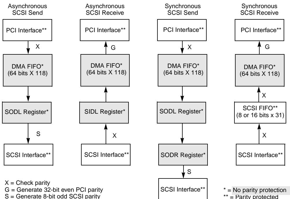
Figure 2.2 Parity Checking/Generation
