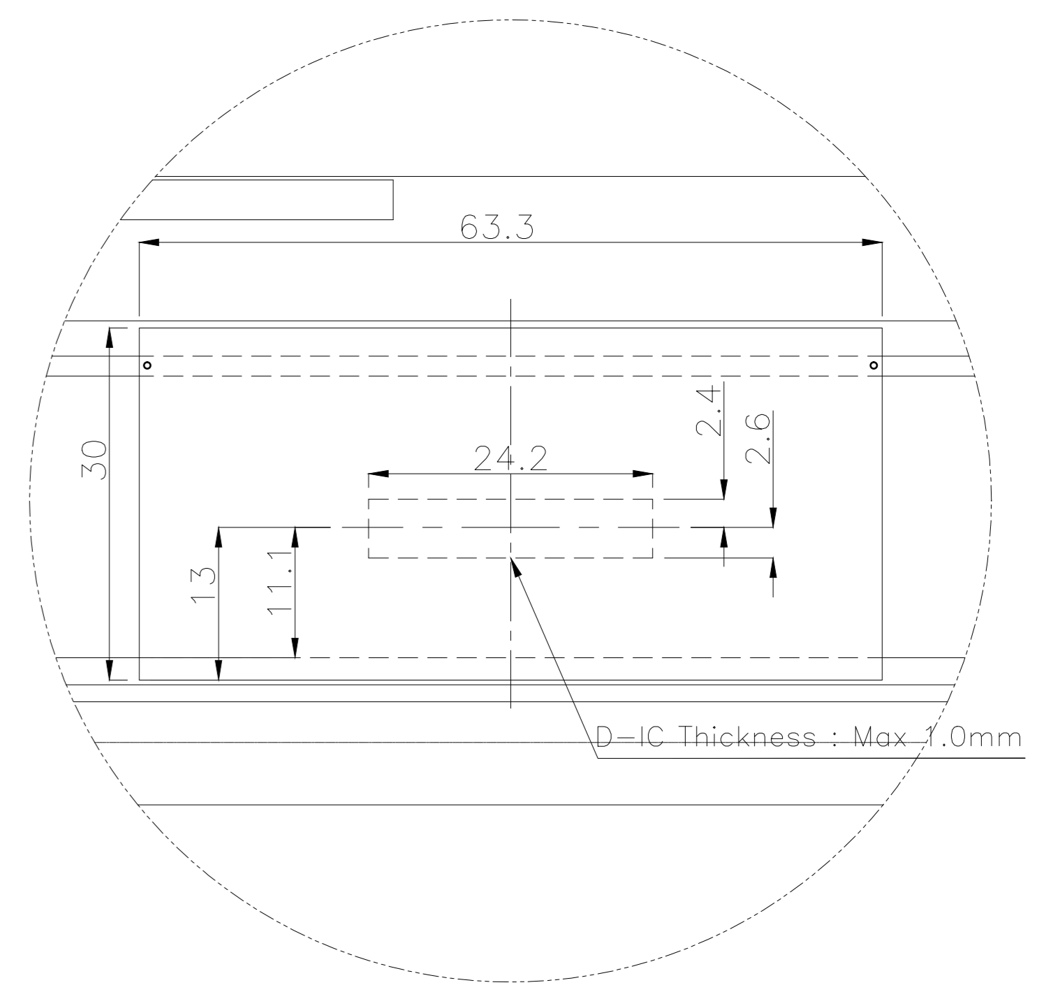
DETAIL "A" (HIDDEN VIEW) (3 : 1)
