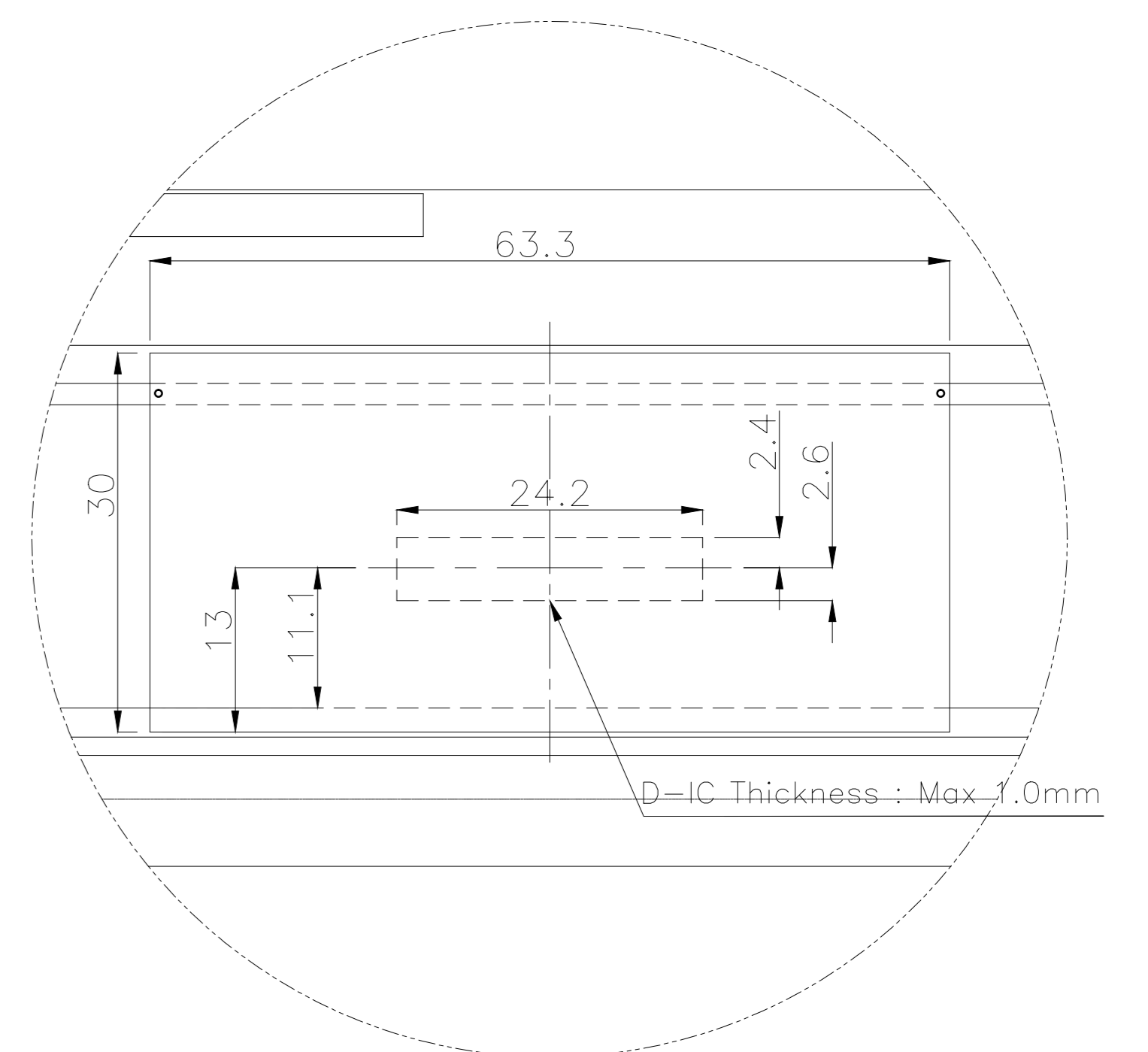
DETAIL "A" (HIDDEN VIEW) (3 : 1)
