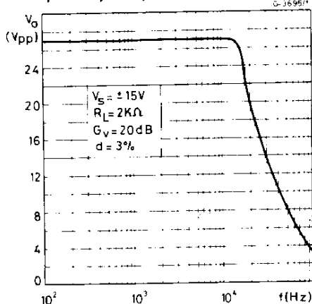
Fig. 7 - Large signal frequency response
