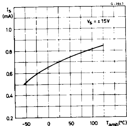
Fig. 2 - Supply current vs. ambient temperature
