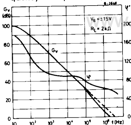
Fig. 4 - Open loop frequency and phase response
