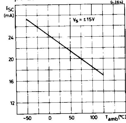
Fig. 3 - Output short circuit current vs. ambient temperature
