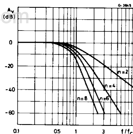
Fig. 11 - Amplitude response
