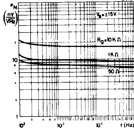
Fig. 9 - Total input noise vs. frequency
