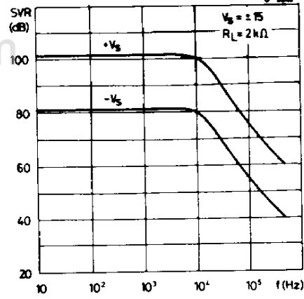
Fig. 6 - Supply voltage rejection vs. frequency
