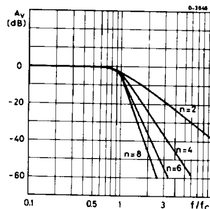
Fig. 10 - Amplitude response
