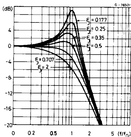
Fig. 14 - Filter response vs. damping factor
