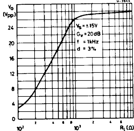
Fig. 8 - Output voltage swing vs. load resistance
