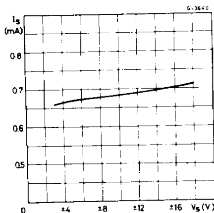
Fig. 1 - Supply current vs. supply voltage
