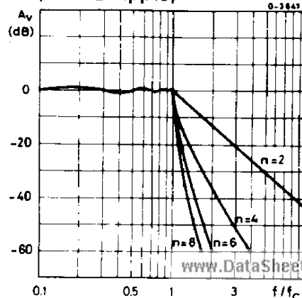
Fig. 12 - Amplitude response ( \pm 1 dB ripple)
