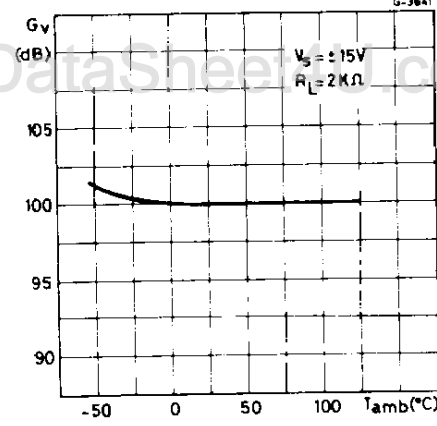
Fig. 5 - Open loop gain vs. ambient temperature
