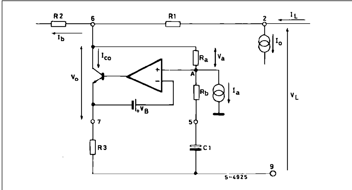
Figure 7 : DC Characteristic.
