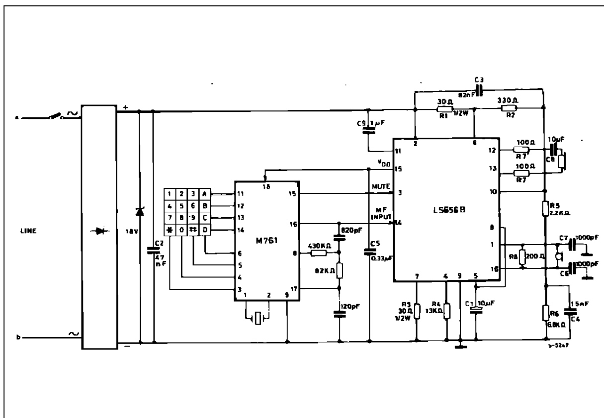
Figure 11 : Application Circuit with Multifrequency (Europe I STD).
