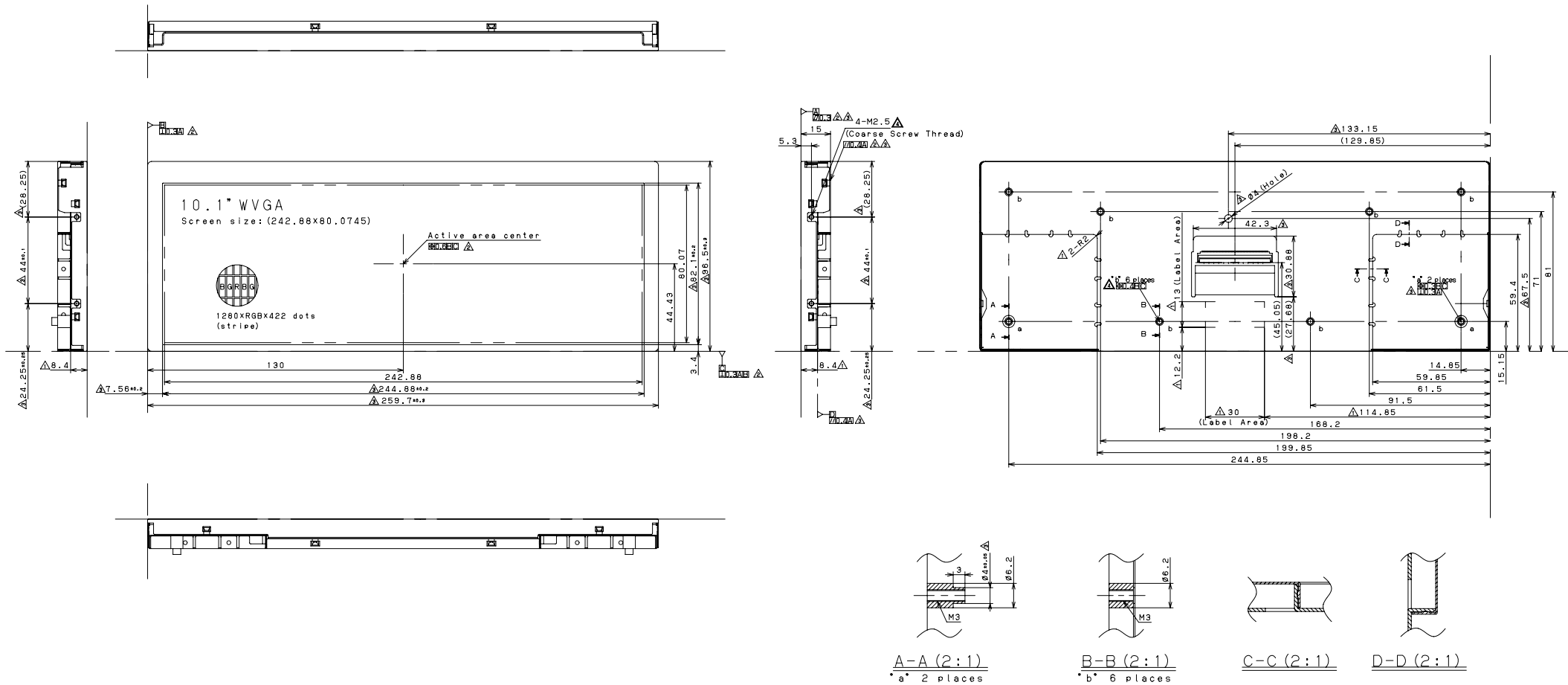
Fig.1 Outline dimensions
