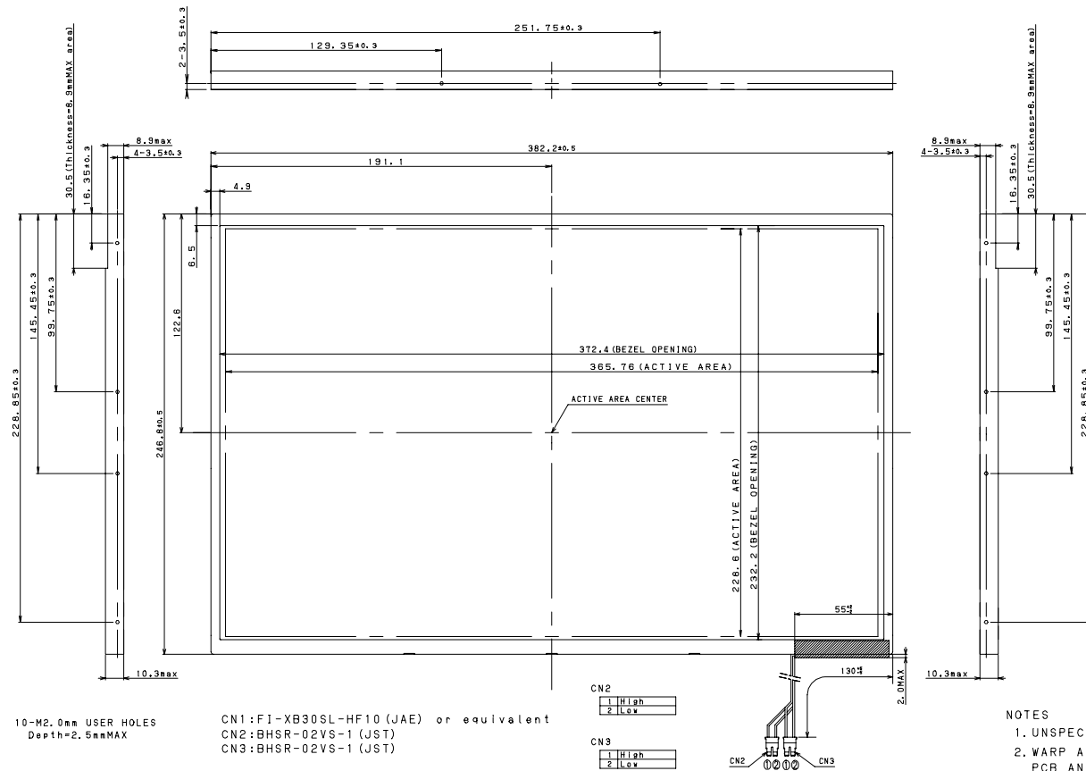
Fig1 . Outline Dimensions
