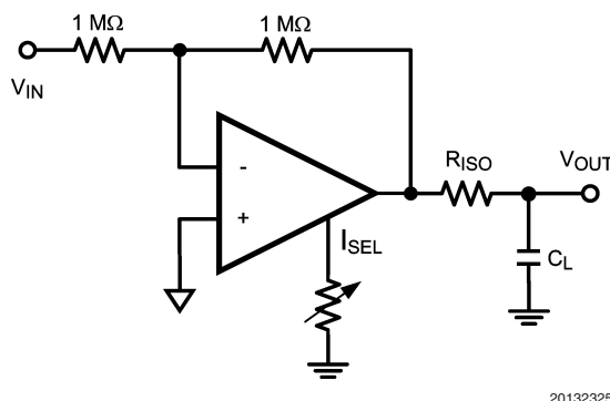
FIGURE 8. Compensation by Isolation Resistor
