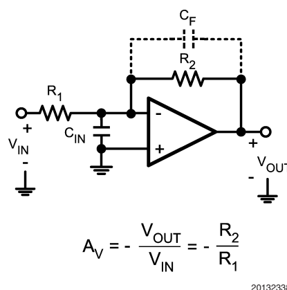
FIGURE 9. Inverting Amplifier
