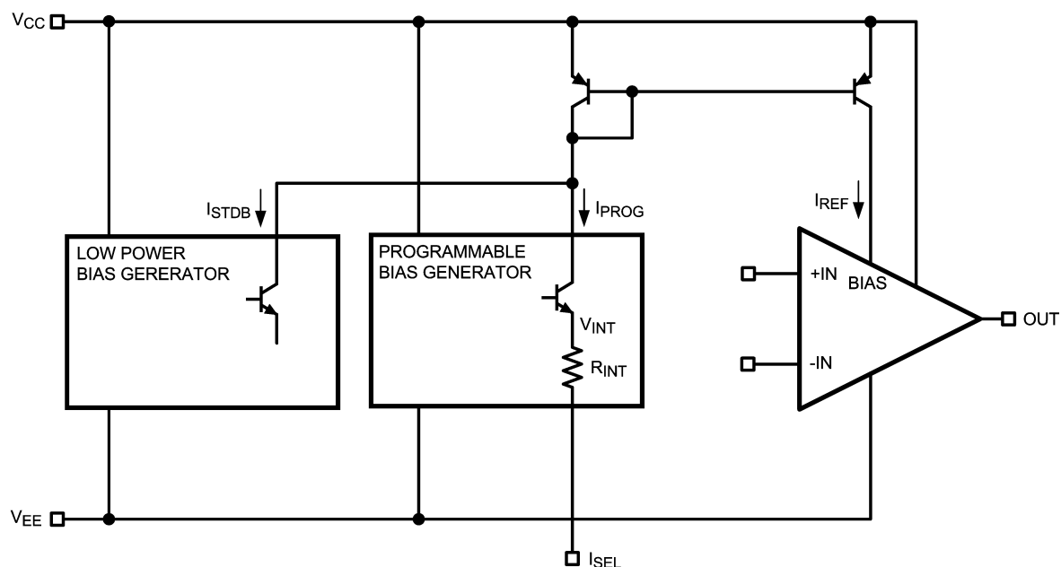
FIGURE 1. Simplified Schematic
