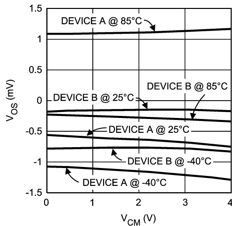
Input Offset Voltage vs. Common Mode Voltage (Full Power Mode)
