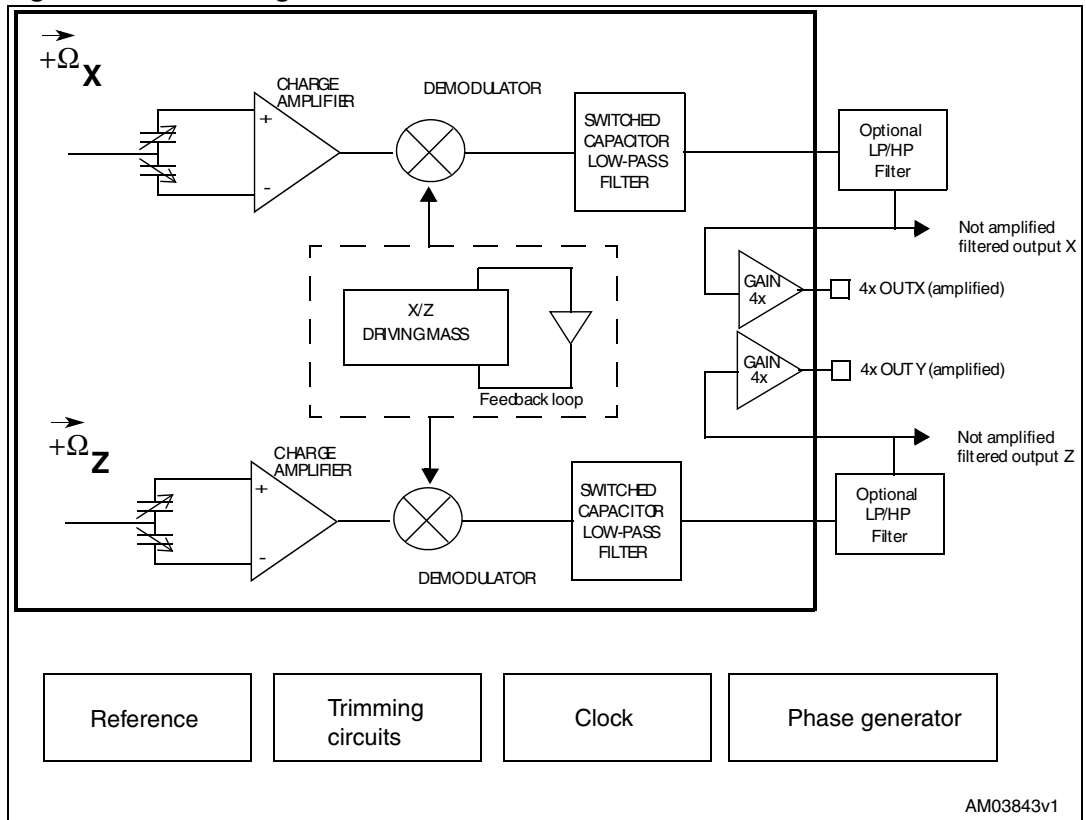
Figure 1. Block diagram
