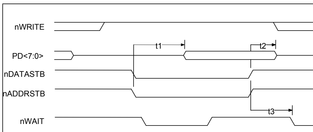
FIGURE 24 – EPP 1.7 DATA OR ADDRESS READ CYCLE
