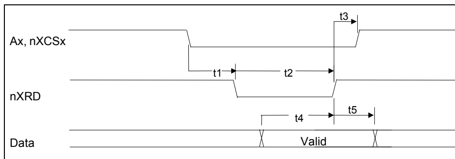
FIGURE 32 – X-BUS READ TIMING
