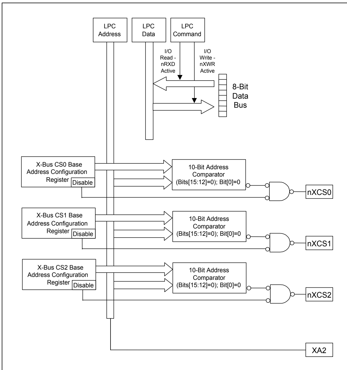
FIGURE 7 – X-BUS INTERFACE, MODE 3
