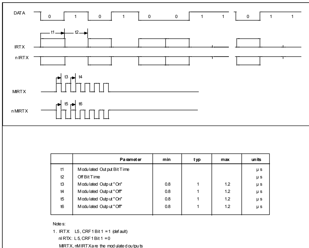
FIGURE 31 – AMPLITUDE SHIFT KEYED IR TRANSMIT TIMING
