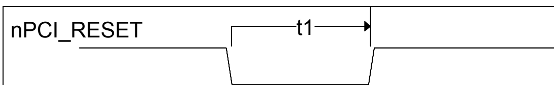
FIGURE 12 - RESET TIMING
