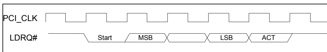
FIGURE 17 – DMA REQUEST ASSERTION THROUGH LDRQ#
