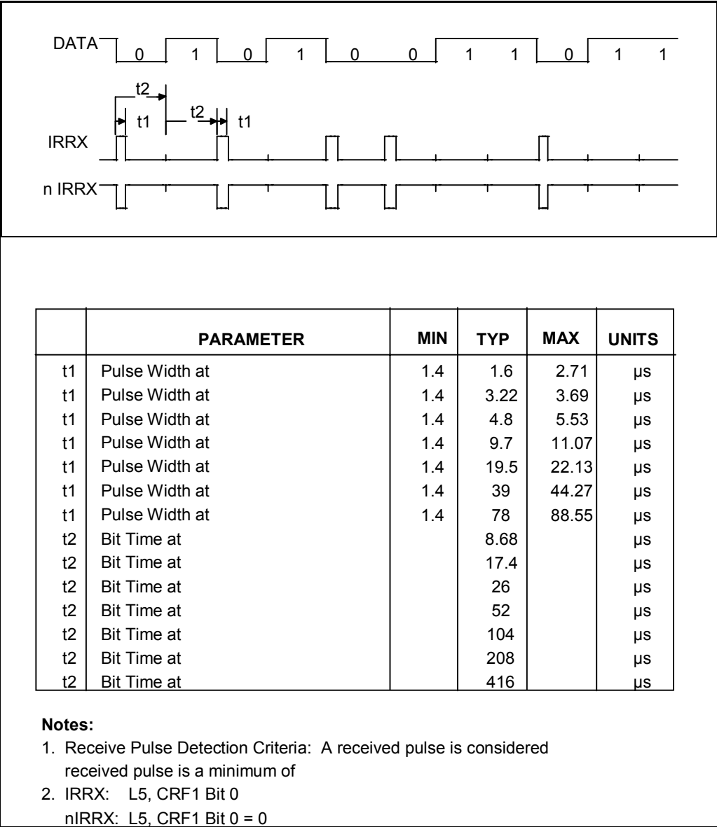
FIGURE 28 - IRDA RECEIVE TIMING
