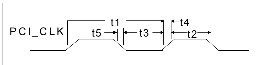
FIGURE 11 – PCI CLOCK TIMING
