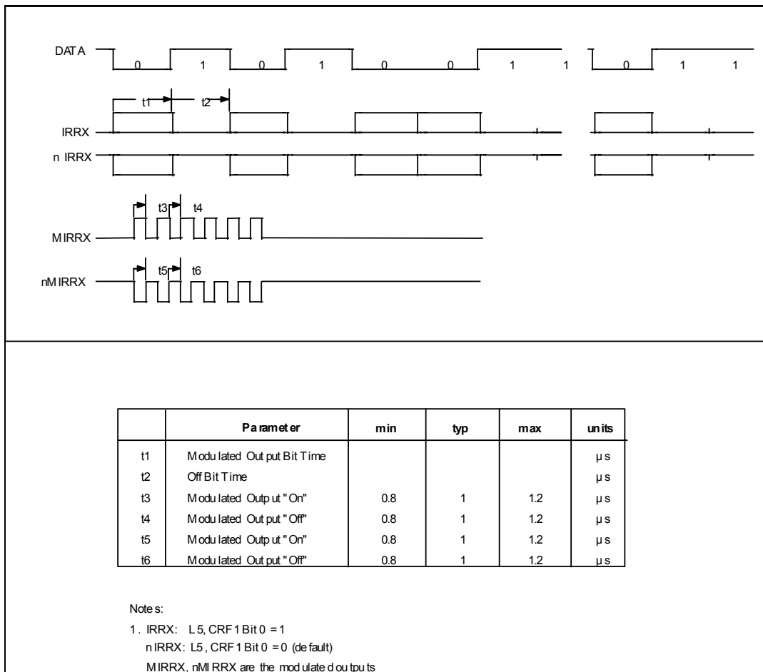
FIGURE 30 – AMPLITUDE SHIFT KEYED IR RECEIVE TIMING
