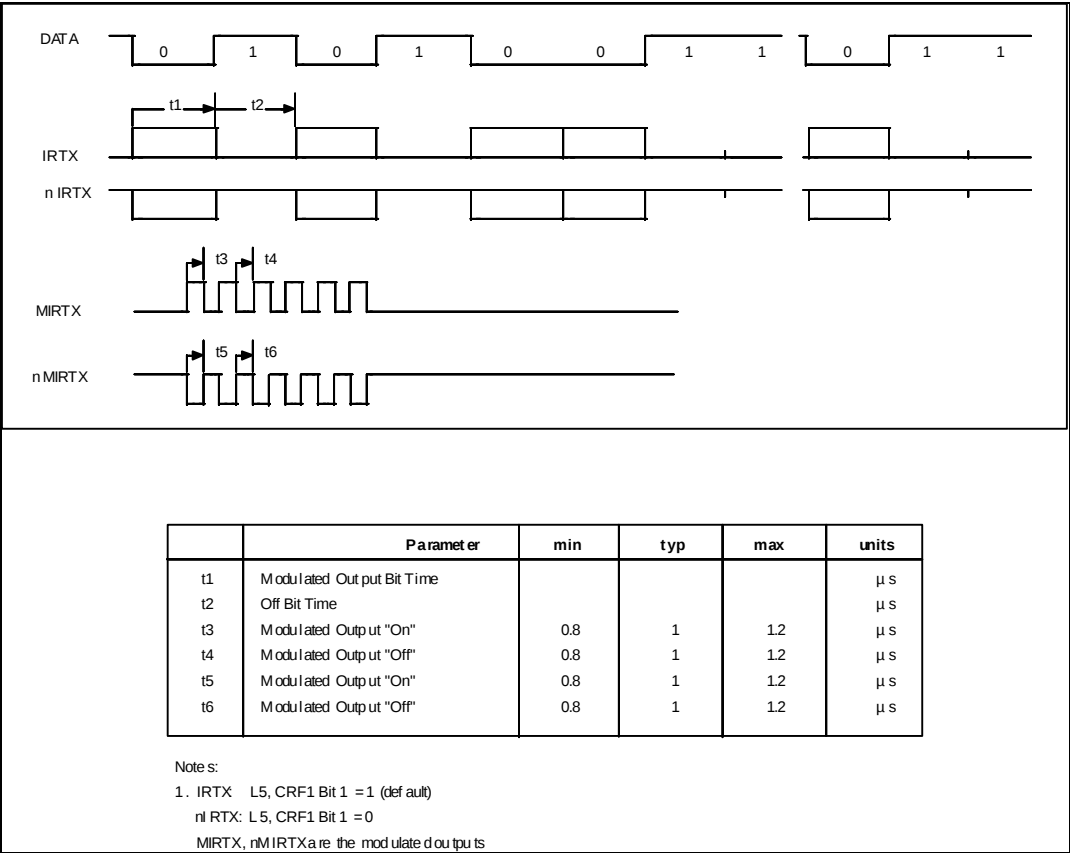
FIGURE 27 - AMPLITUDE SHIFT KEYED IR TRANSMIT TIMING
