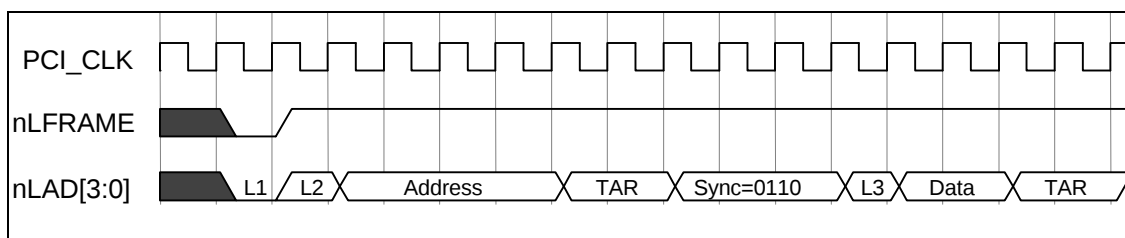
FIGURE 12 – I/O READ
