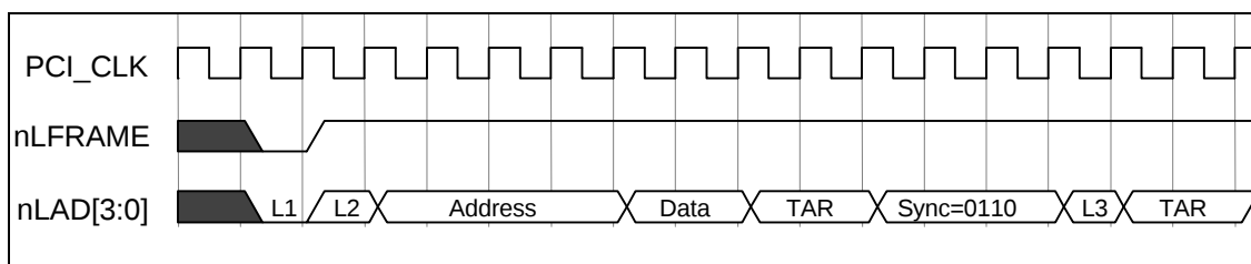
FIGURE 11 – I/O WRITE
