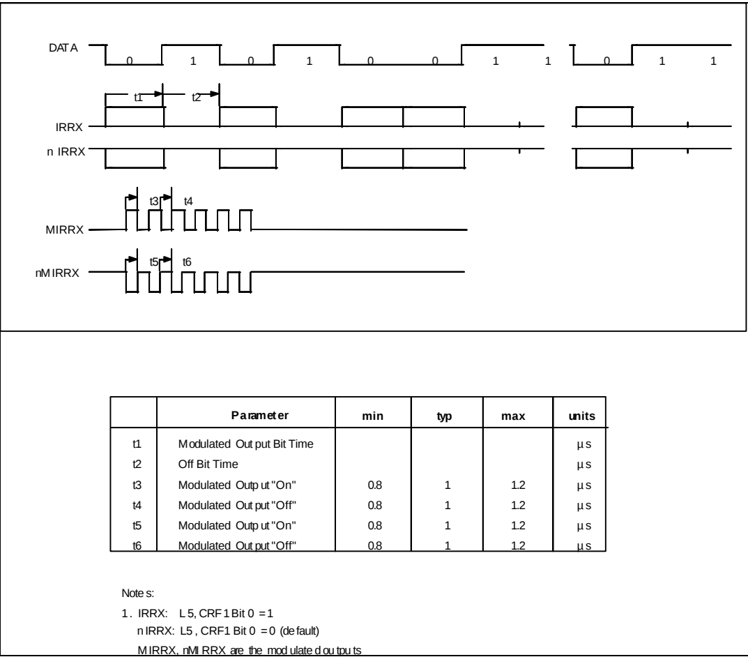
FIGURE 26 - AMPLITUDE SHIFT KEYED IR RECEIVE TIMING
