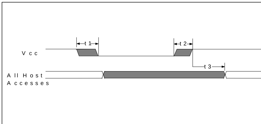
FIGURE 7 - POWER-UP TIMING
