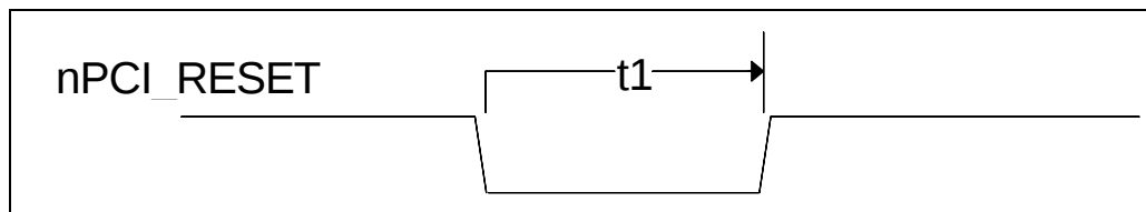
FIGURE 8C - RESET TIMING
