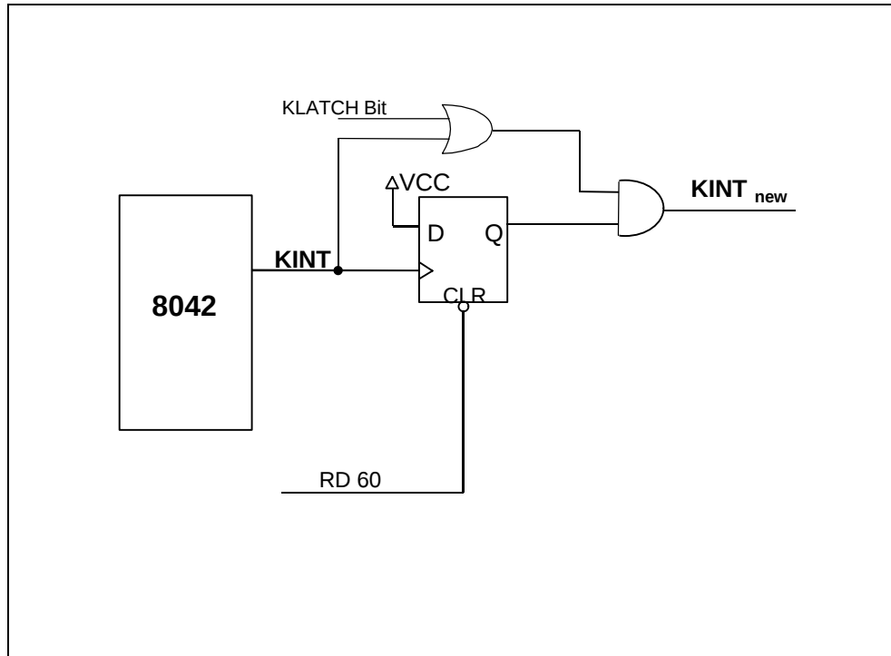
FIGURE 3 - KEYBOARD LATCH
