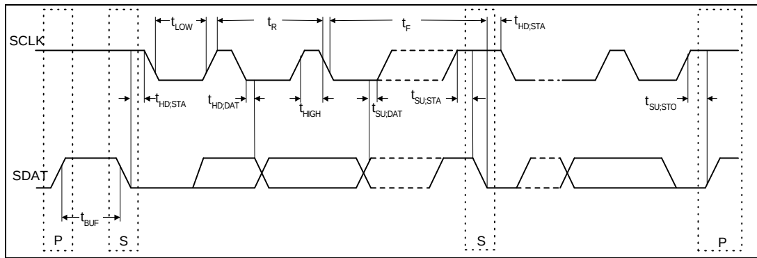
FIGURE 28 - SMBUS TIMING
