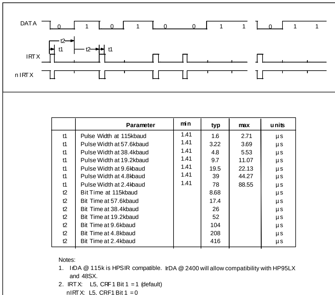
FIGURE 22 - IRDA TRANSMIT TIMING
