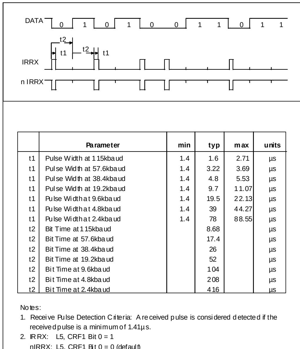
FIGURE 21 - IRDA RECEIVE TIMING
