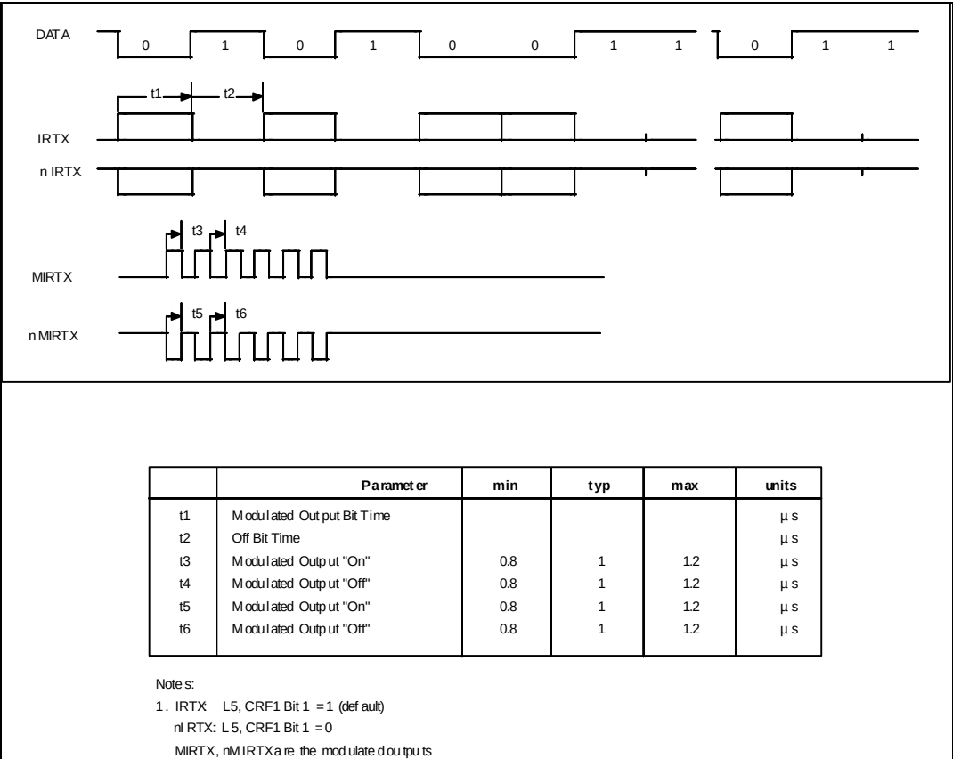
FIGURE 24 - AMPLITUDE SHIFT KEYED IR TRANSMIT TIMING
