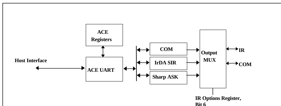
FIGURE 1 – IR COMPONENTS/BLOCK DIAGRAM
