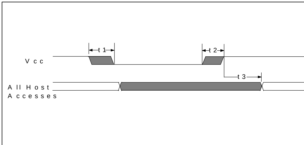
FIGURE 3 - POWER-UP TIMING
