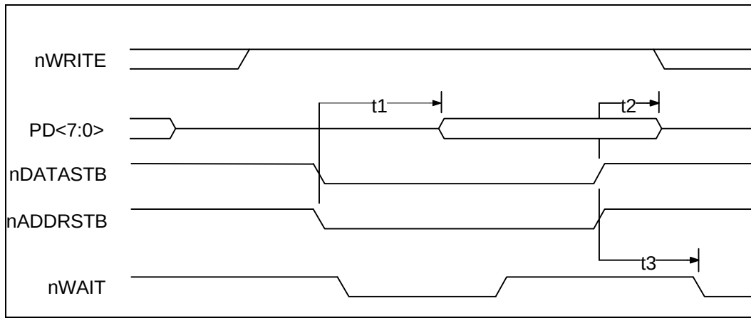
FIGURE 17 – EPP 1.7 DATA OR ADDRESS READ CYCLE
