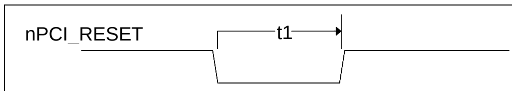
FIGURE 5 - RESET TIMING
