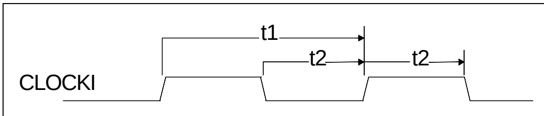
FIGURE 4 - INPUT CLOCK TIMING
