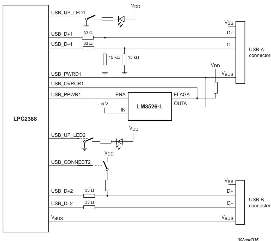
Fig 23. LPC2388 USB OTG port configuration: USB port 2 device, USB port 1 host
