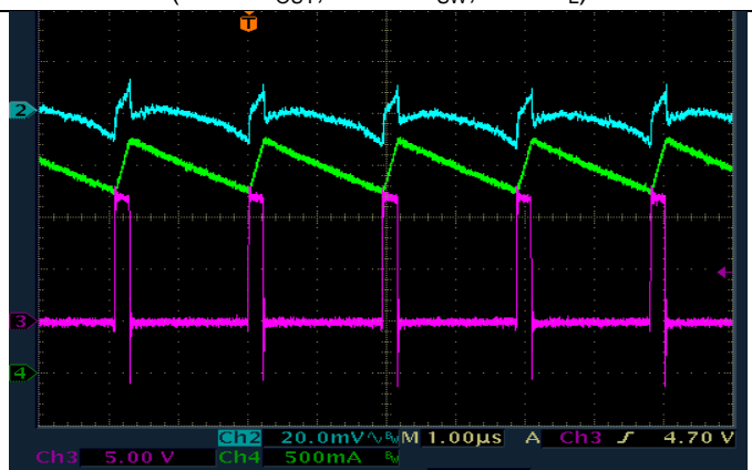
V_{IN}=12V , V_{OUT}=1.2V , I_{OUT}=2.0A (CH2= V_{OUT} , CH2= V_{SW} , CH3= I_L )
