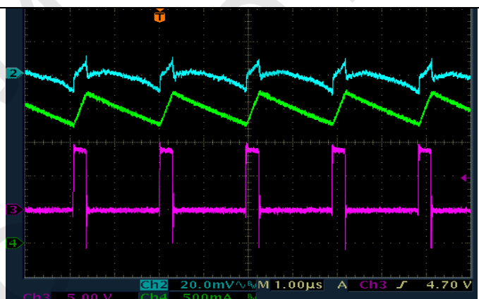
V_{IN}=9V , V_{OUT}=1.2V , I_{OUT}=2.0A (CH2= V_{OUT} , CH2= V_{SW} , CH3= I_L )
