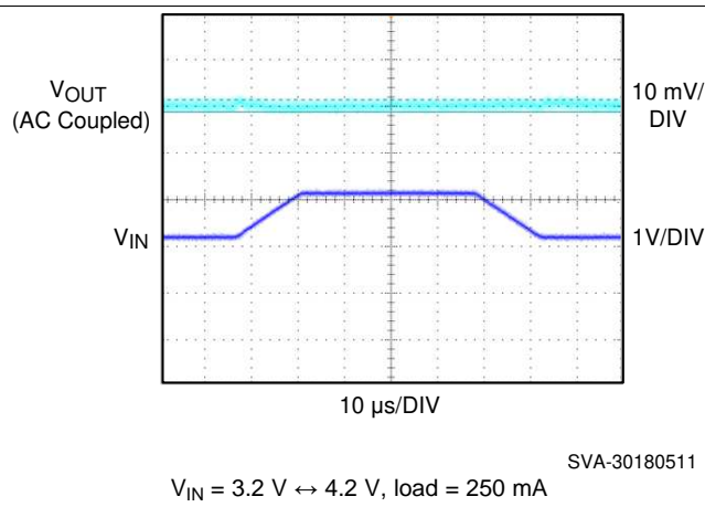
Figure 10. Line Transient
