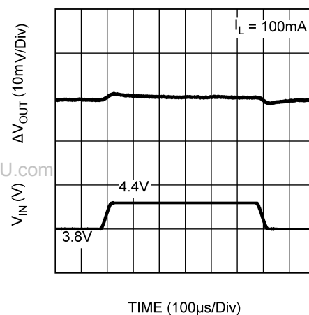
Line Transient
