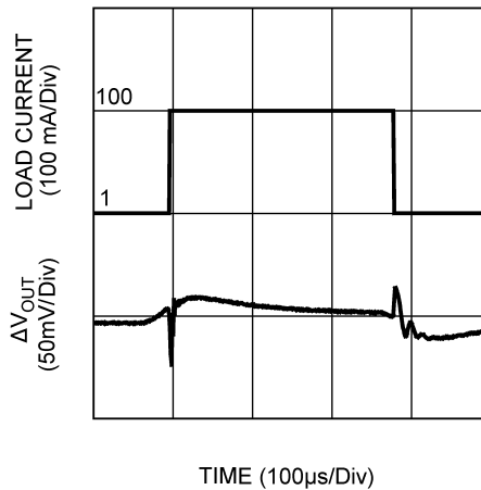
Load Transient
