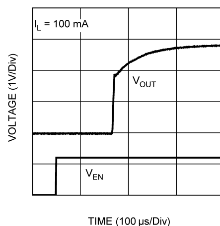
Enable Start-up Time, ( I_L = 100mA , V_{OUT} = 2.8V )
