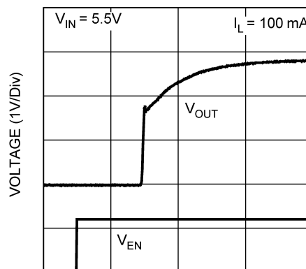
Enable Start-up Time, ( I_L = 100mA , V_{OUT} = 2.8V )
