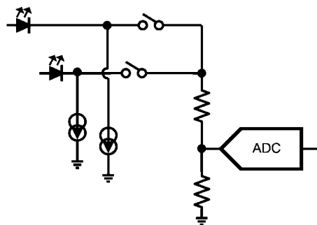
Principle of LED Connection to ADC
