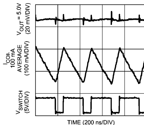
Boost Typical Waveforms with 100 mA Load
