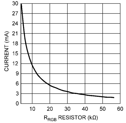
Output Current vs R_{\text{RGB}} (Current Sink Mode)
