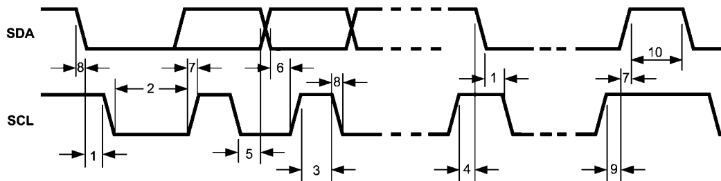
I 2 C Timing Diagram
